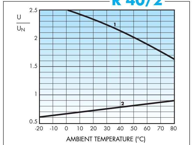
Operating range (DC sensitive type) vs ambient temperature. 1 - Max coil voltage permitted 2 - Min pick-up voltage with coil at ambient temperature
