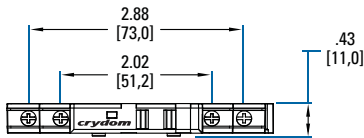
For DRxxx06
