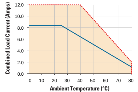
DRDxxD06
