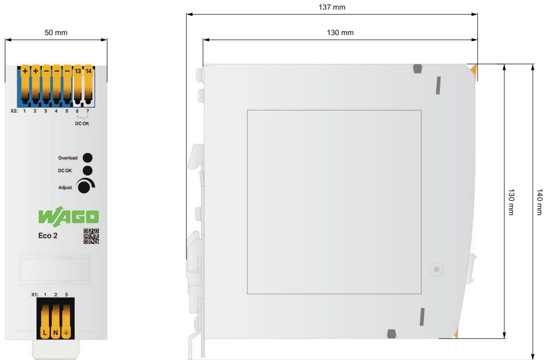
Figure 7: Dimensions
