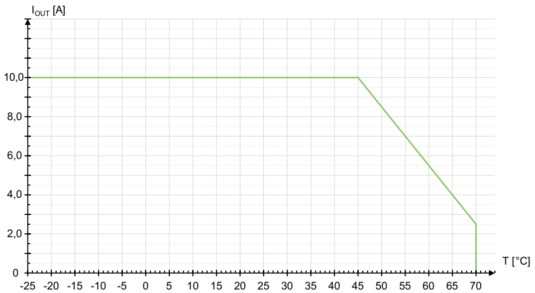
Figure 10: Derating (Temperature-Dependent)
