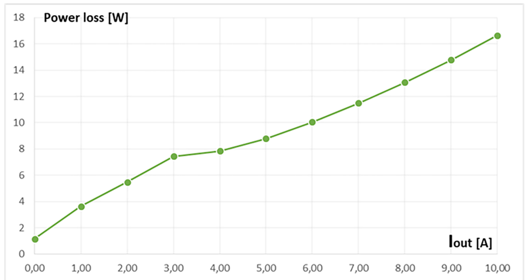
Figure 9: Power loss at 230 VAC
