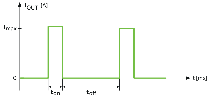
Figure 11: Hiccup-Mode
