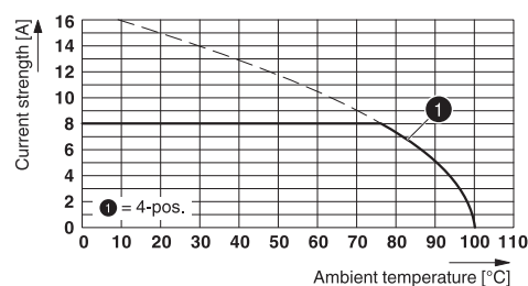
Type: MC 1,5/ 4-ST-3,81 with MCDB 1,5/ 4-G1-3,81 P20 THR TR
