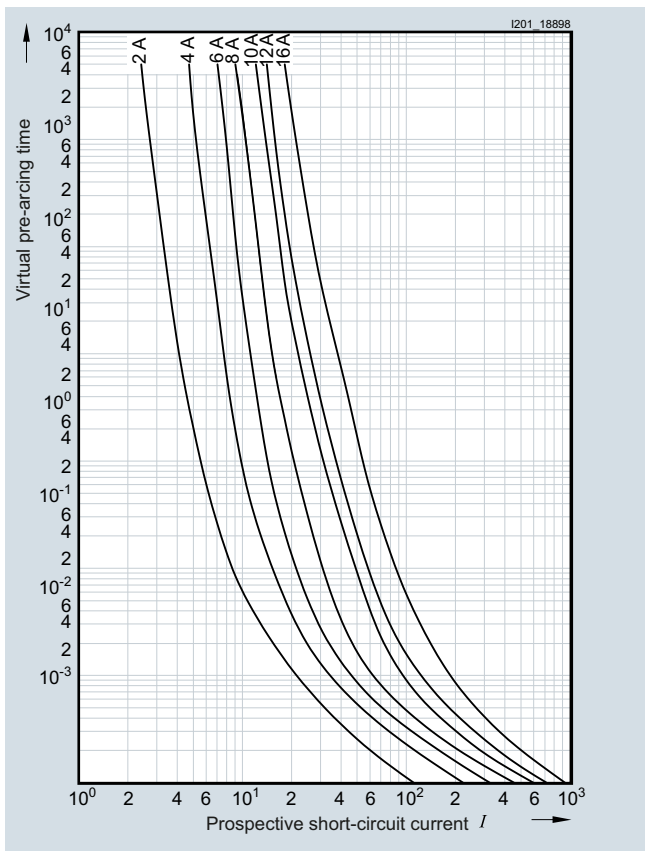
Time/current characteristics diagram
