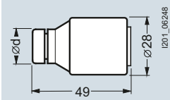
5SB3, 5SB4
