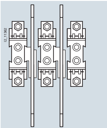
3 LV HRC fuse bases, 1P
