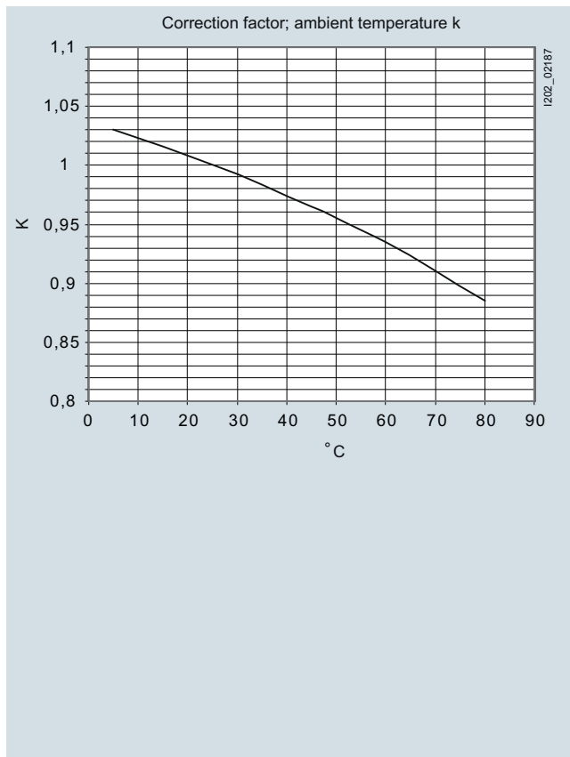
Characteristic curves diagram Correction factor Ambient temperature
