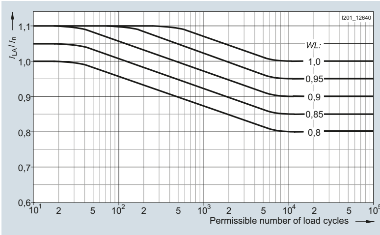
Waveform of the varying load factor WL for load cycles
