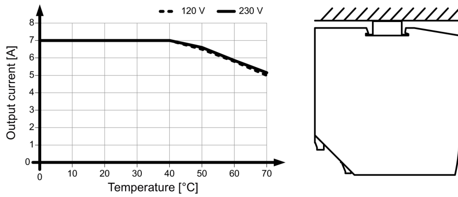
Figure 4-32 Mounting position (5)
