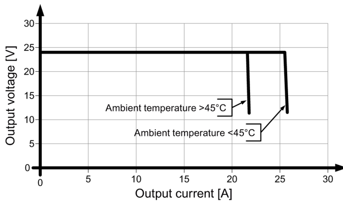
Figure 6-6 Output characteristic 6EP1336-2BA10
