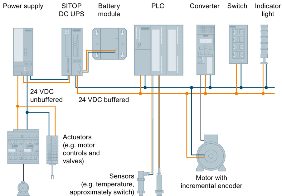
Figure 9-7 24 V buffering to maintain communication, signaling functions, sensor measured values and position values
