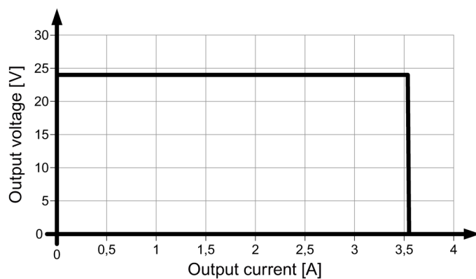
Figure 6-3 Output characteristic 6EP1332-2BA20
