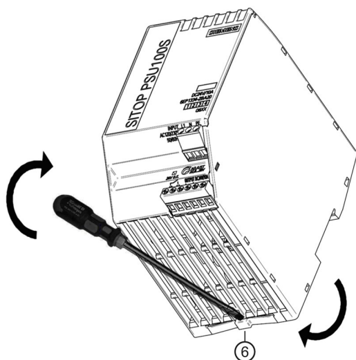
Figure 3-1 Removal
