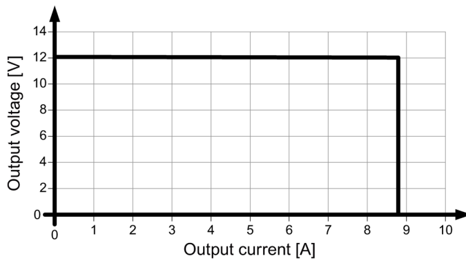
Figure 6-7 Output characteristic 6EP1322-2BA00
