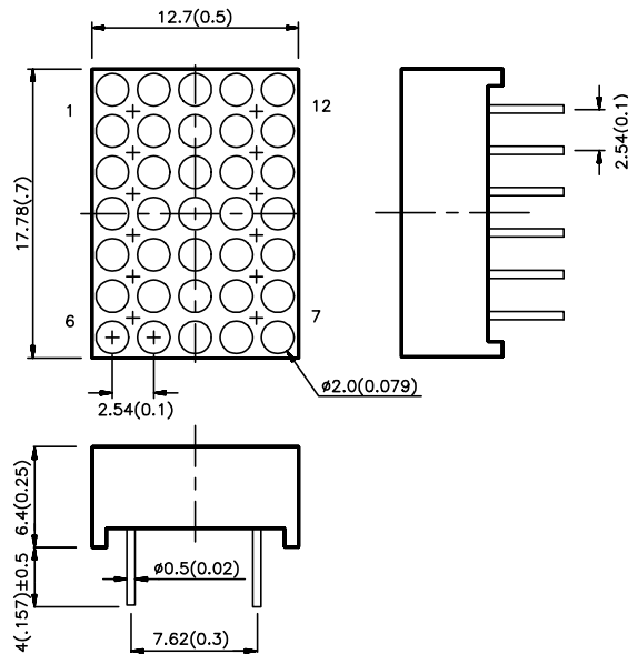
Package Dimensions
