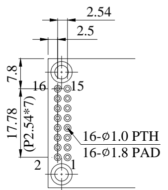
PIN DETAIL SCALE 1/1
