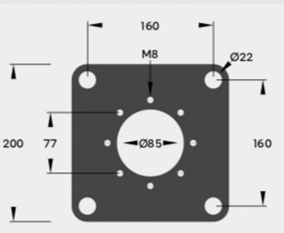
Adapter plate
