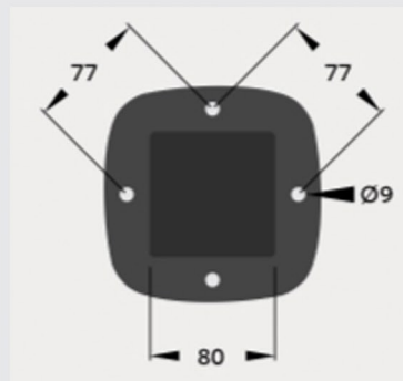
Post base plate
