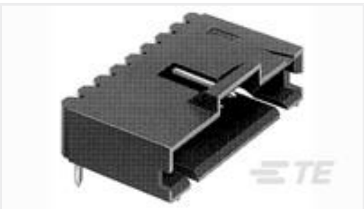
TE Part #6-103635-2 13 MTE HDR SRRA LTCH.100CL LF
