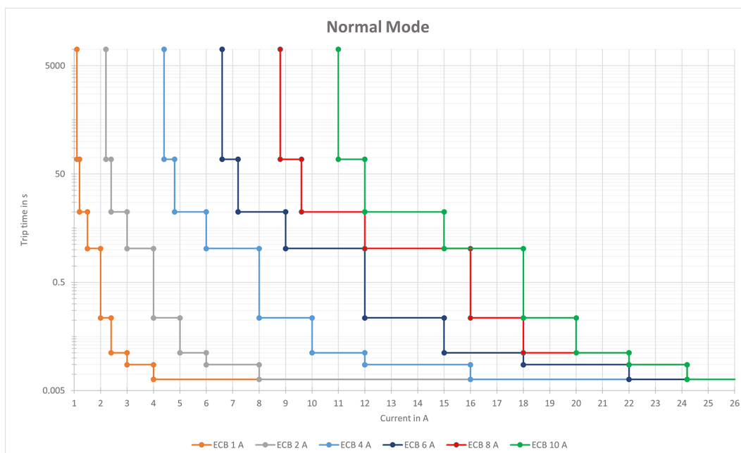
Figure 5: Tripping curve "Normal Mode"
