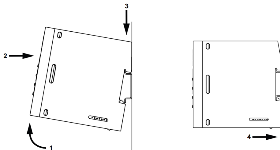
Figure 8: Mounting the product on the DIN rail
