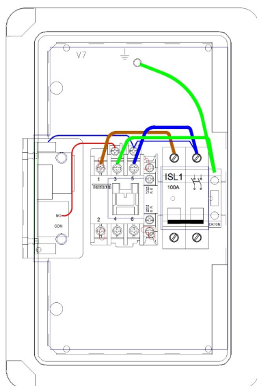
IP-EVCP-T
