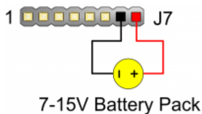
Figure 3.2 Arty A7 Battery Pack Connection
