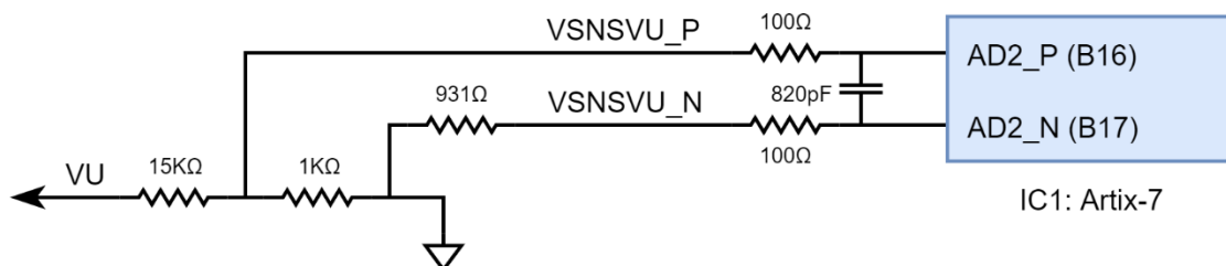
Figure 3.1.1 Monitoring External Supply Voltage
