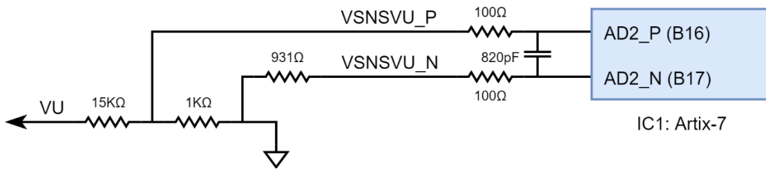
Figure 3.3.1 5V Supply Power Monitoring
