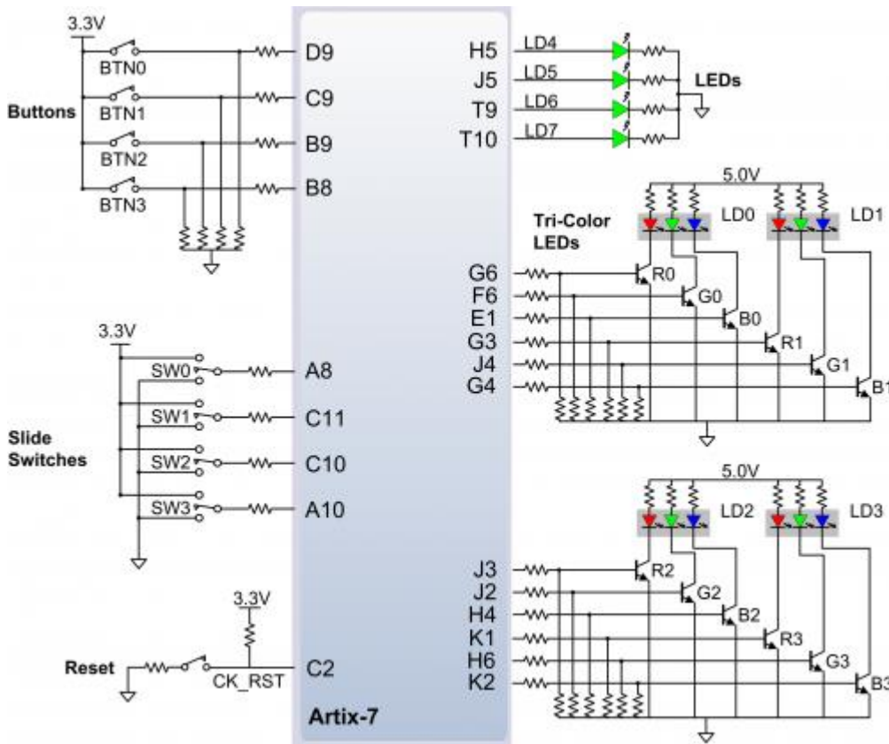
Figure 9.1 Arty A7 GPIO
