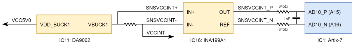
Figure 3.2.1 FPGA Core Supply Current Monitoring
