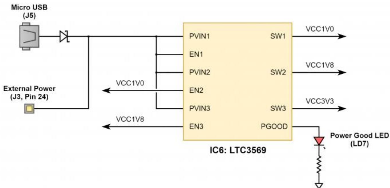
Figure 1.1 Power Supply
