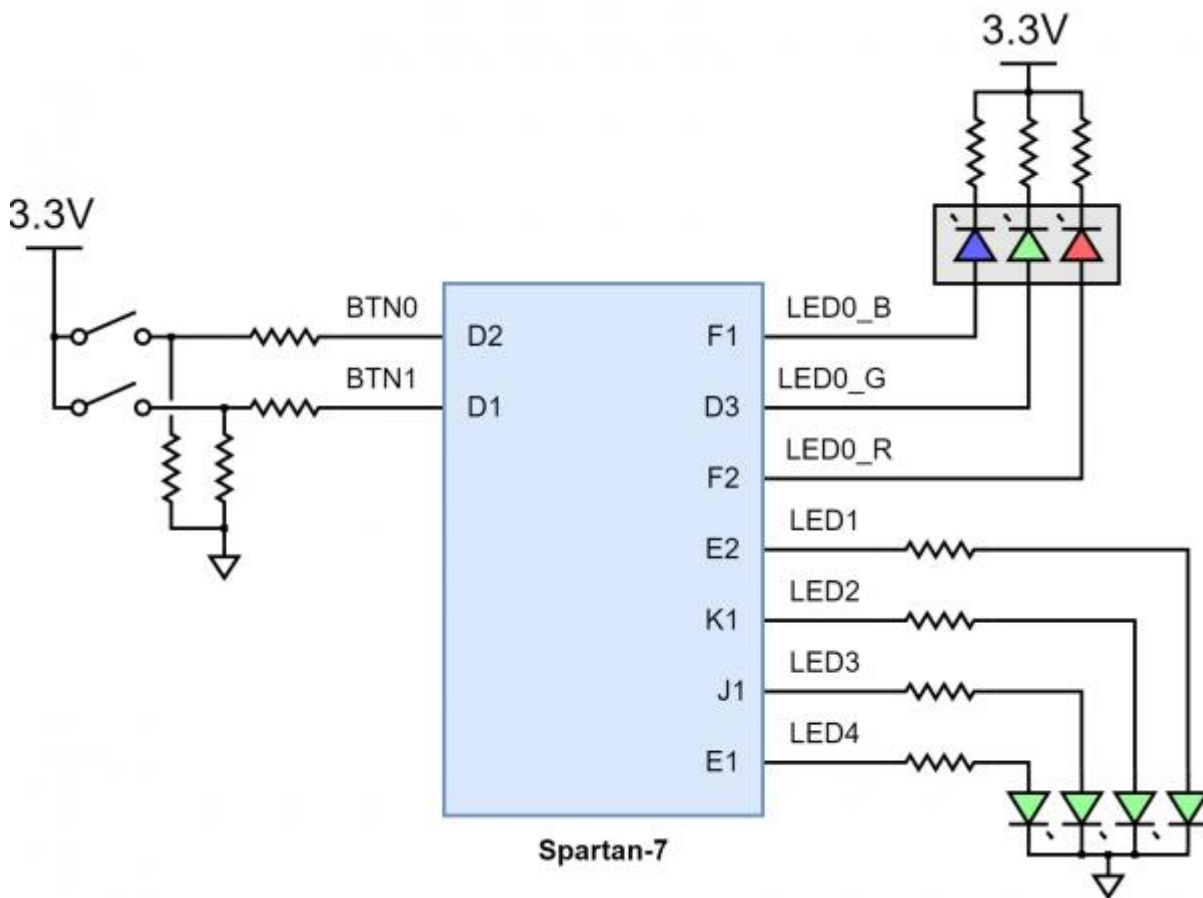
Figure 6.1 Cmod S7 Basic I/O
