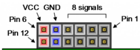
Figure 8.1 Pmod Diagram
