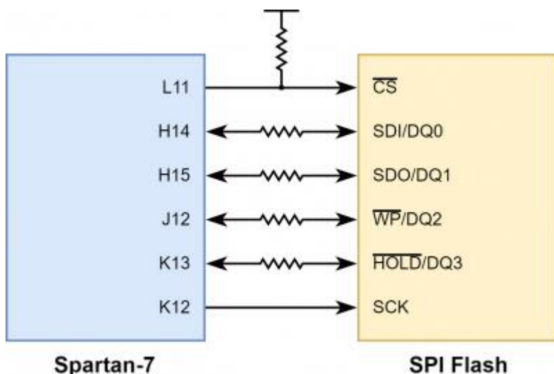
Figure 3.1 Flash Interface
