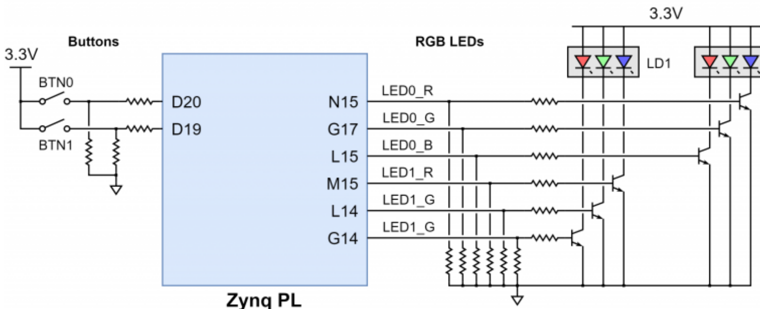
Figure 11.1. Cora Z7 Basic I/O
