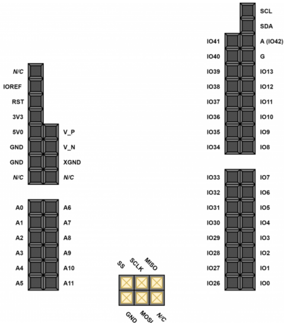
Shield connector pin diagram.
