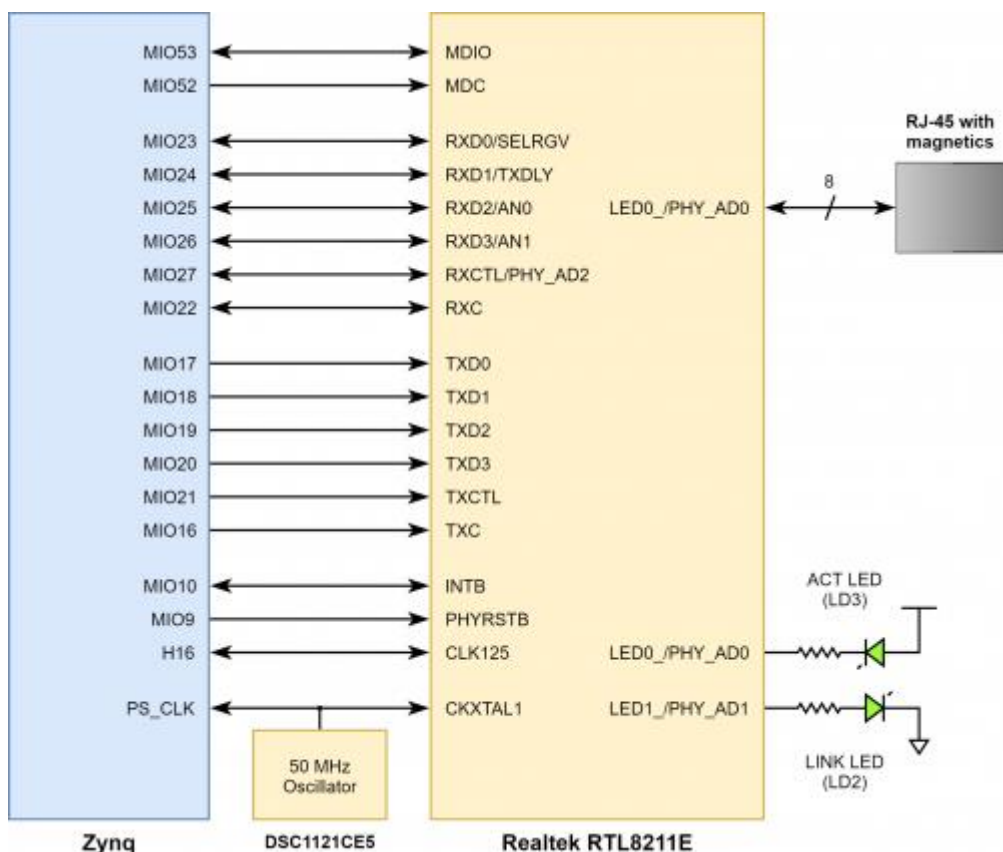
Figure 8.1. Ethernet PHY
