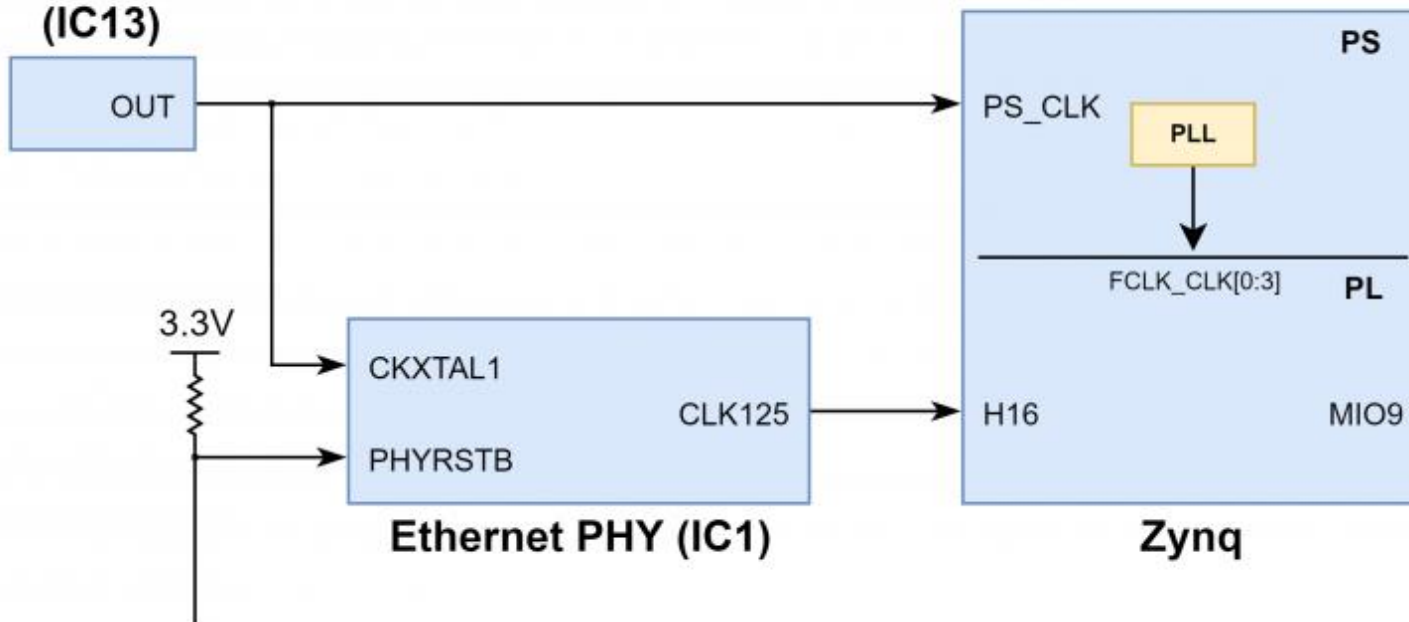
Figure 9.1. Cora Z7 Clocking
