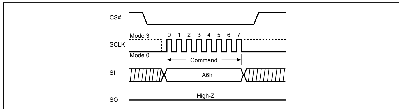
Figure 61. SPB Lock Bit Set (SPBLK) Sequence
