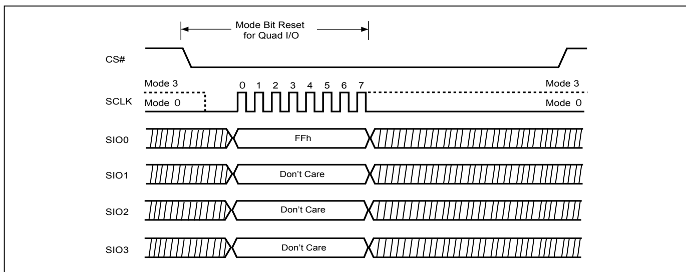
Figure 37. Performance Enhance Mode Reset for Fast Read Quad I/O (SPI Mode)
