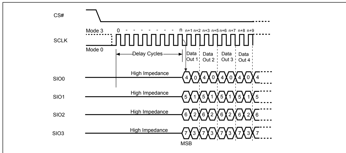
Figure 40. Fast Boot Sequence (QE bit =1)
