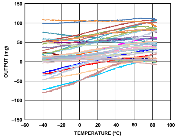
Figure 13. X-Axis Zero g Offset vs. Temperature—45 Parts Soldered to PCB, V_s = 2.5 V
