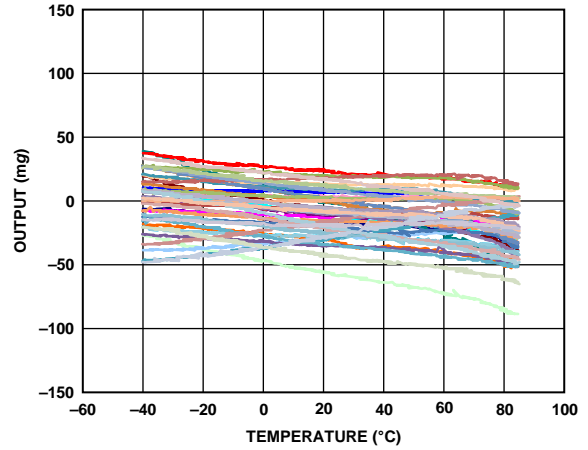
Figure 14. Y-Axis Zero g Offset vs. Temperature—45 Parts Soldered to PCB, V_s = 2.5 V
