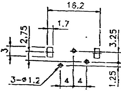
HOLE LAYOUT (SIDE VIEW)
