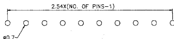
Recommended P.C.Board Layout
