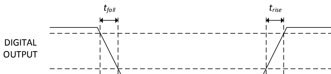
Figure 2: Digital IO Characteristics
