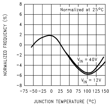
Oscillator Frequency
