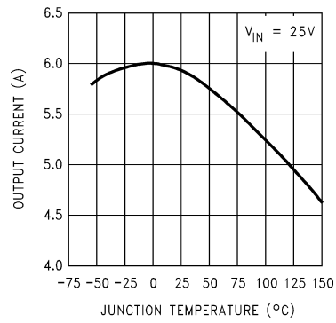
Current Limit
