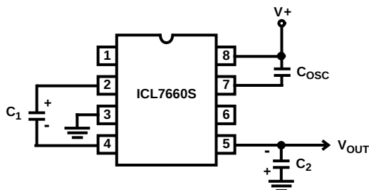
FIGURE 19. LOWERING OSCILLATOR FREQUENCY
