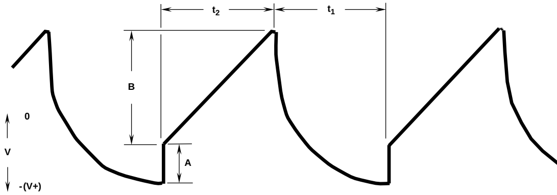
FIGURE 15. OUTPUT RIPPLE
