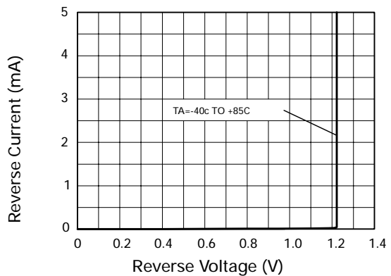
Reverse Characteristics
