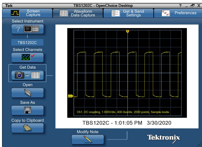
Figure 17: OpenChoice desktop
