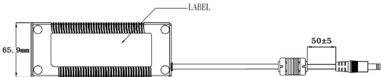
BOTTOM-VIEW
