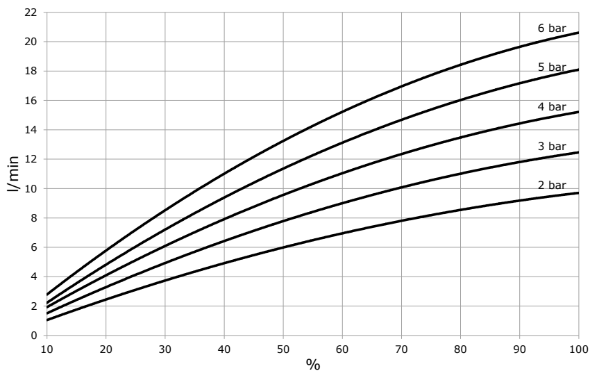
Typical airflow
